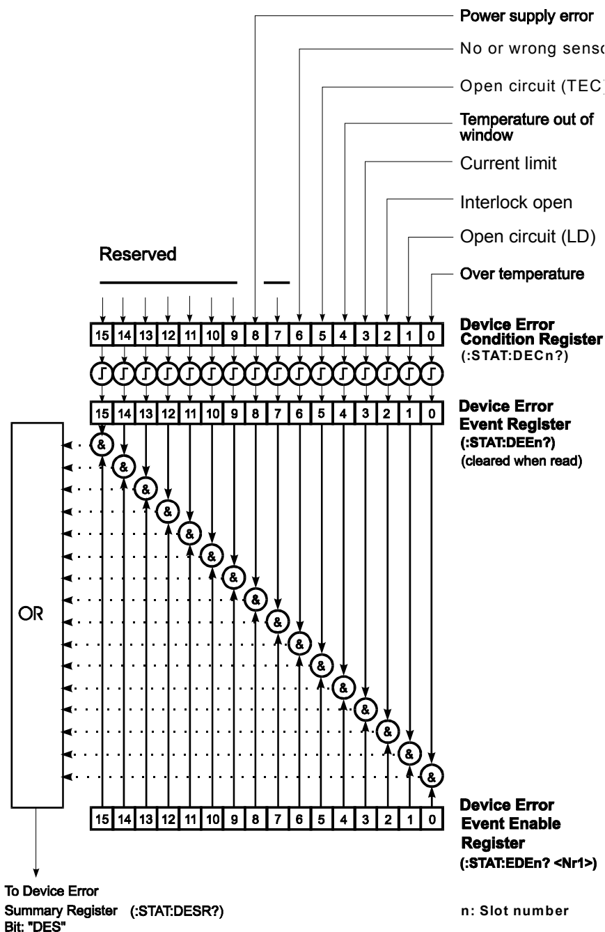
Figure 11 The ITC8xxx device error registers DEC, DEE and EDE
